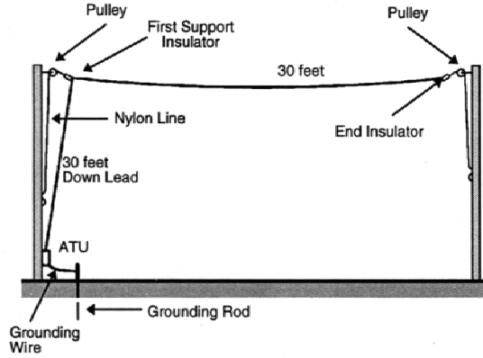
Figure 2-5. Inverted "L" Antenna
