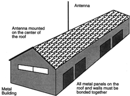
Figure 2-9. Practical Ground Using a Metal Building
